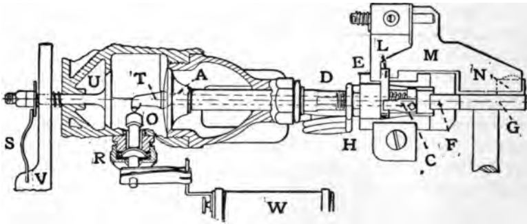
FIG. 176.—The Duryea Primary Spark Ignition Apparatus. A is the exhaust valve; D, the exhaust valve stem; T, the stem of the sparker hammer, journaled in the stem; E, the exhaust slide; F, roller at end of E; G, the rotating exhaust cam; H, exhaust valve spring; J, a clamp fixed in position by a set screw; M, pivoted lift that trips the hammer, L, operated by roller; N, beside the exhaust cam, knocking the sparker, T, away from the insulated plug, O. U is the inlet valve; V, the throttle slide; S, spring controlling the opening of U; W, the spark coil; R, the metal union nut, clamping O in place.
